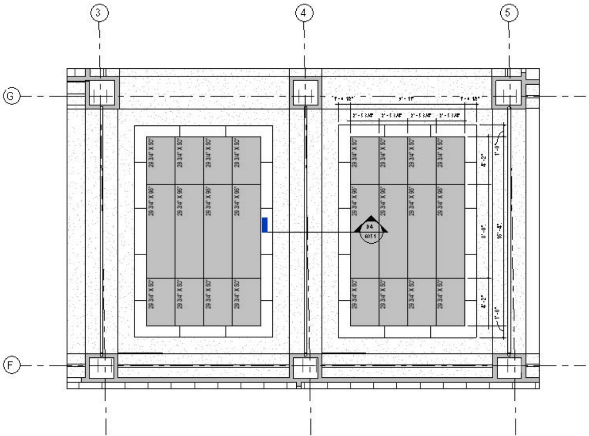
D1 SECOND FLOOR - CEILING PANEL LAYOUT 835 1 1/8" = 1'-0"
